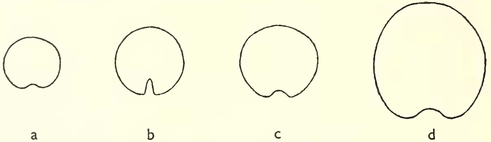
TEXT-FIG. 1. Cross-sections of Belemnopsis guards.
